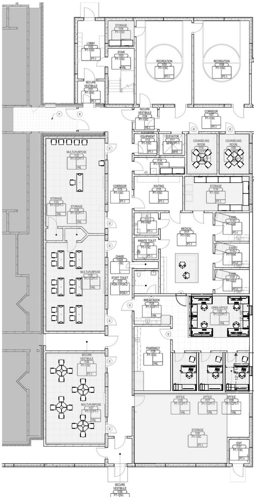
FURNITURE PLAN OVERALL 1ST FLOOR
