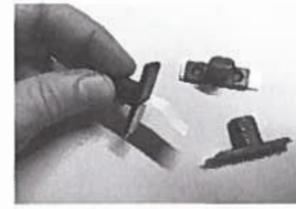
Peel & Stick Alignment feature on Twist Lock Fasteners with Screws
